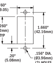
PANEL CUTOUT DETAIL
